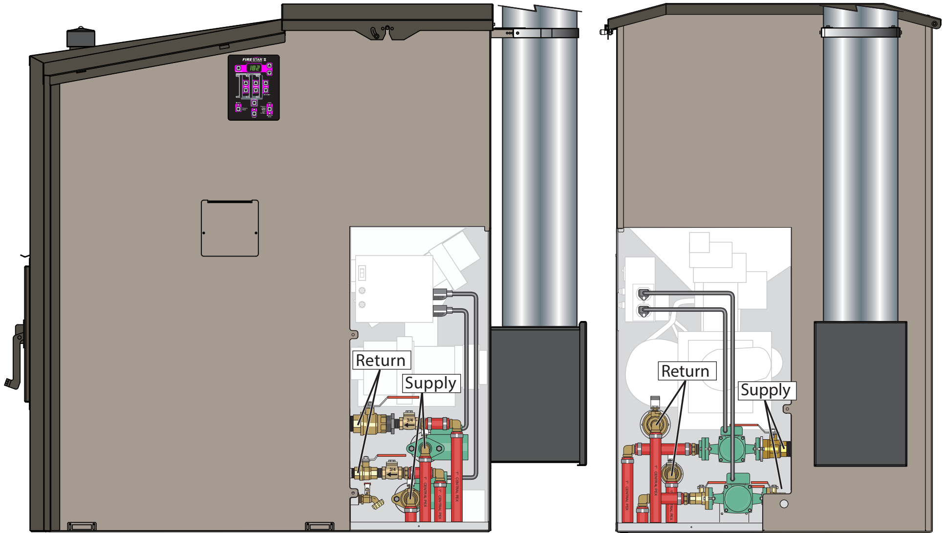
Side View
